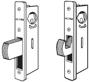
Standard Bolt Cylinder Sold Separately
